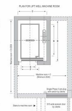
DIMENSIONAL DETAILS : HOSPITAL LIFT
