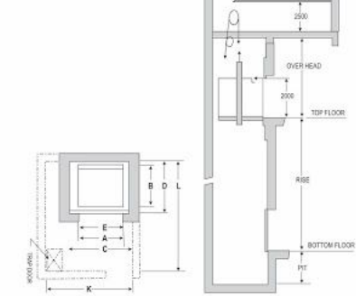
HOISTWAY MACHINE ROOM SIZES
